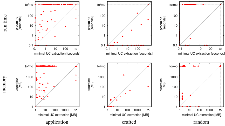
Fig. 22 Comparison of minimal UC extraction with TRP++ (x-axis) and with procmine (y-axis) in terms of run time (in seconds) and memory (in MB) separated by categories application , crafted , and random . TRP++ produced only time outs but no memory outs. procmine produced both. TRP++ likely explores a larger search space during minimization and possibly produces more fine-grained UCs than procmine in that it computes a minimal UC in LTL as a syntax tree according to Def. 11, whereas procmine computes a minimal set of unsatisfiable top-level conjuncts.
